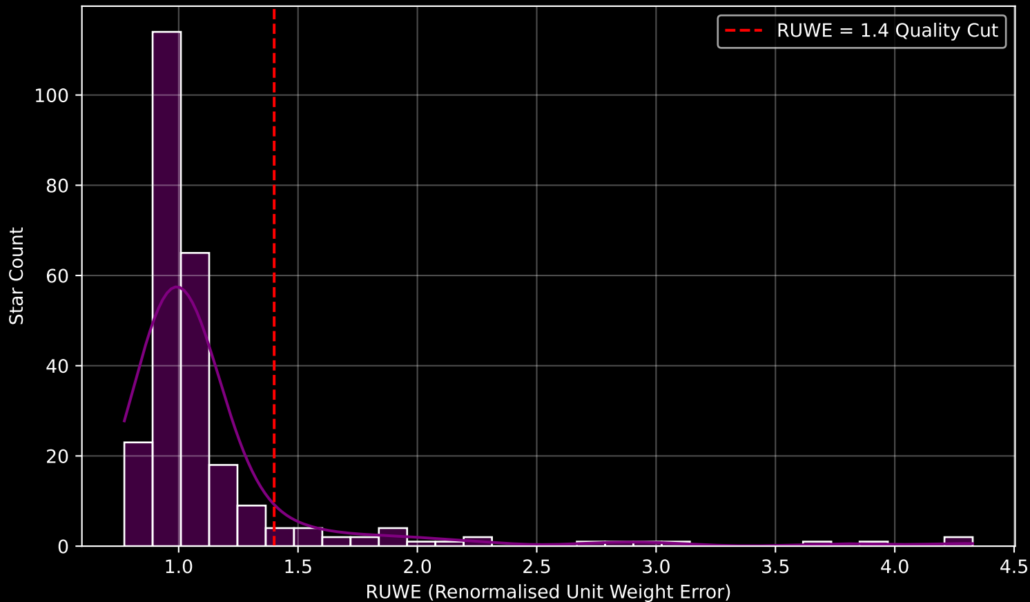
GALAH DR4 Field [501] RUWE Distribution (n= 257)
