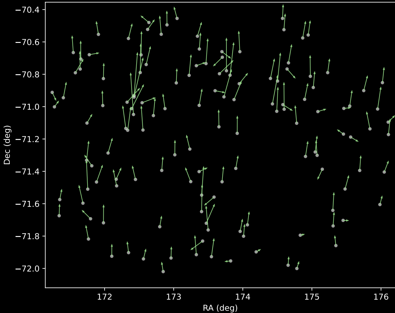
GALAH DR4 Cluster 5 Proper Motion Vectors (n=134)
