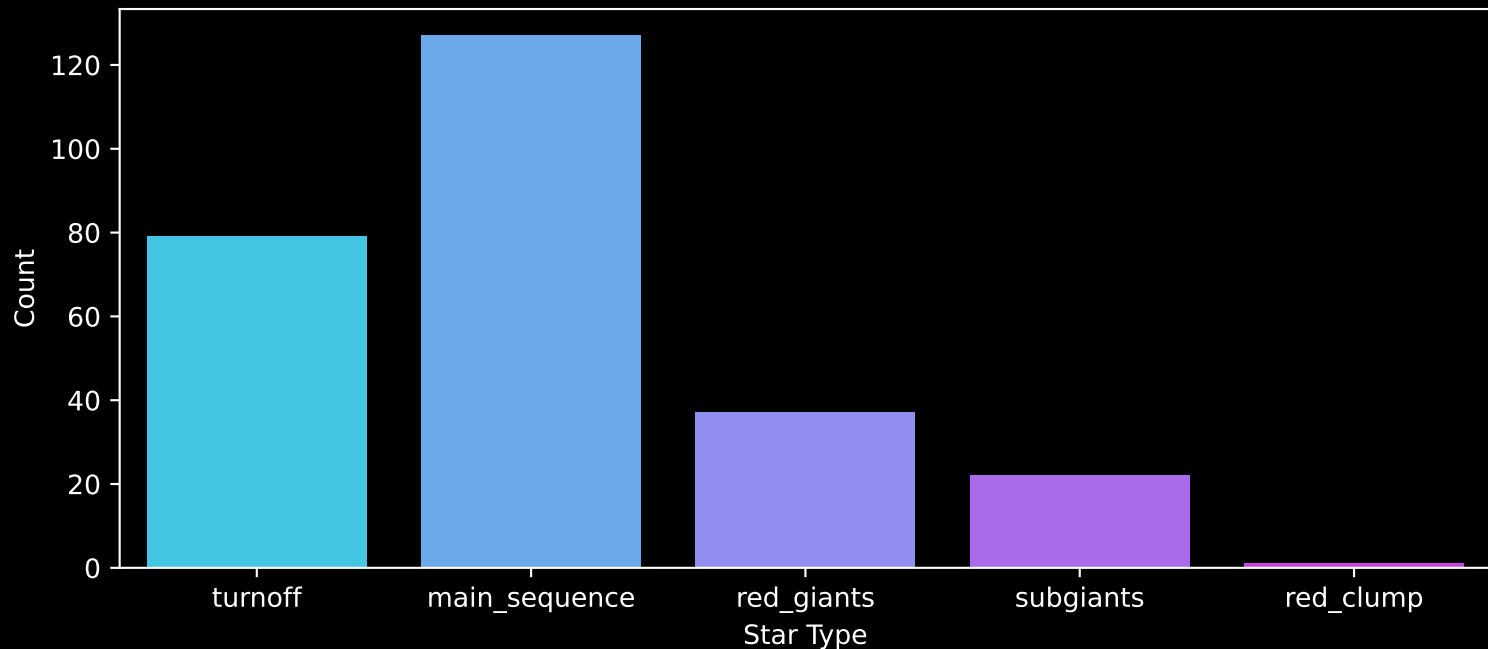
GALAH DR4 Field: [501] Count plot of Star Type
